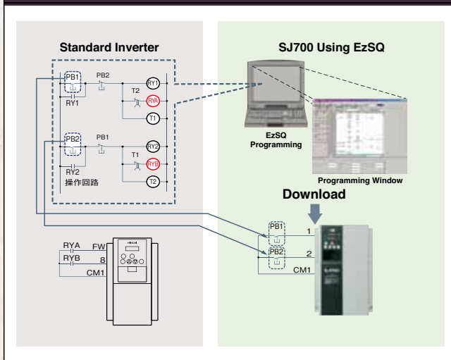
Typical Example - Replacing External Relay Circuit
